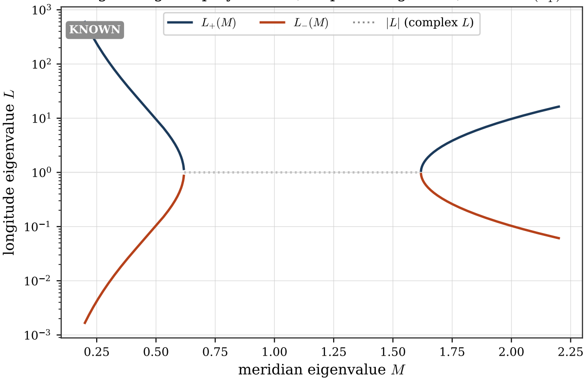
Figure-eight A-polynomial (Cooper--Long, 1996) from \text{Fix}(T_1^2)
