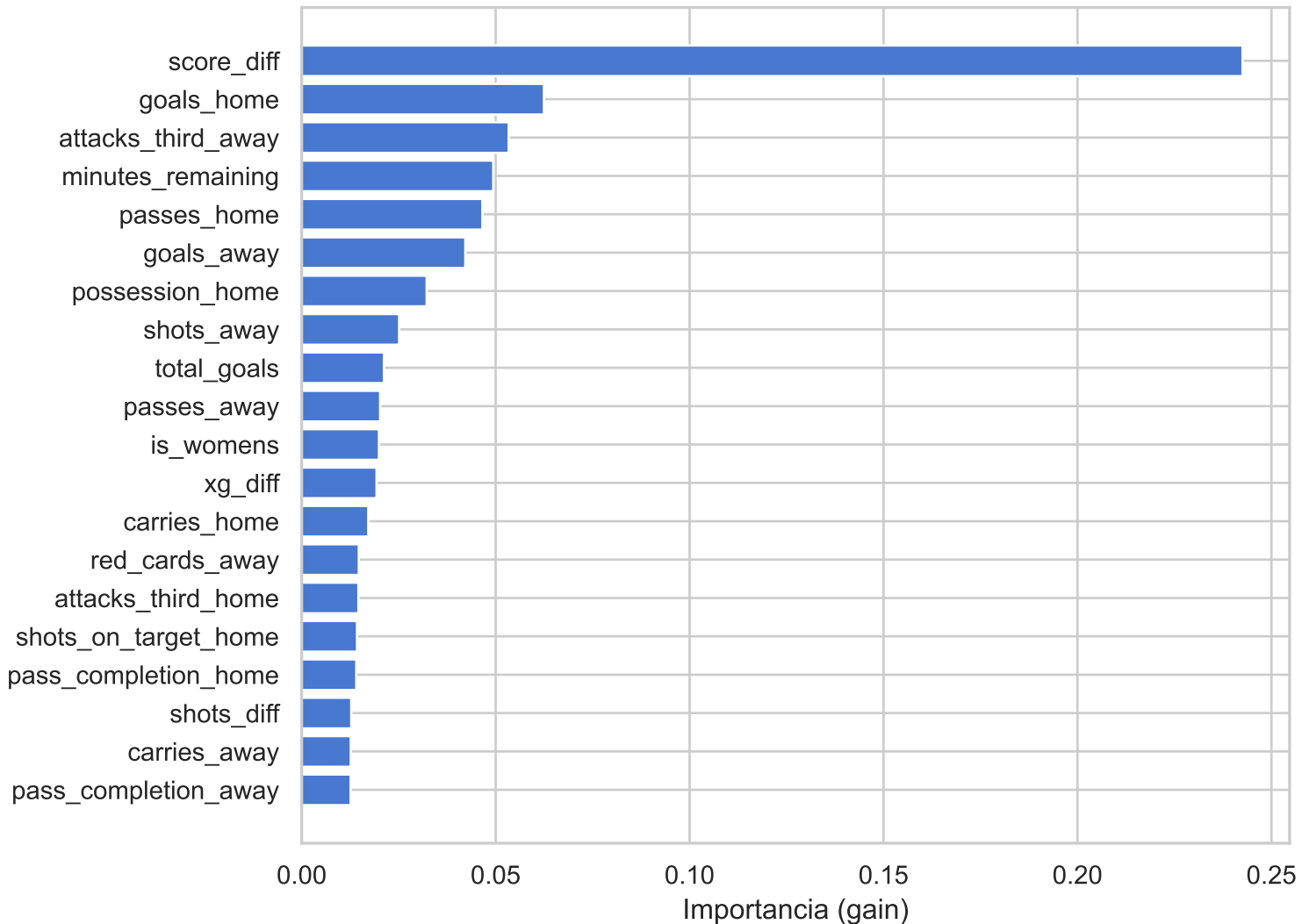
Top 20 features — XGBoost
