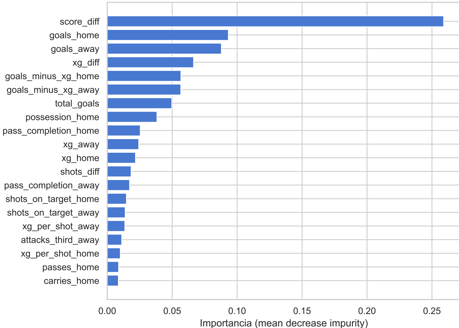
Top 20 features — Random Forest
