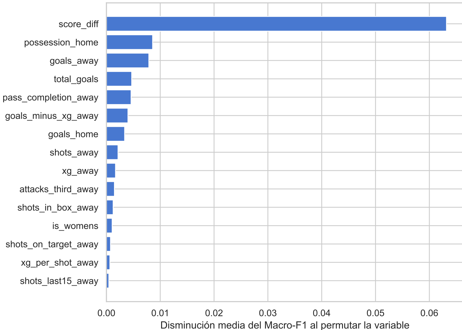
Permutation Importance - Random Forest
