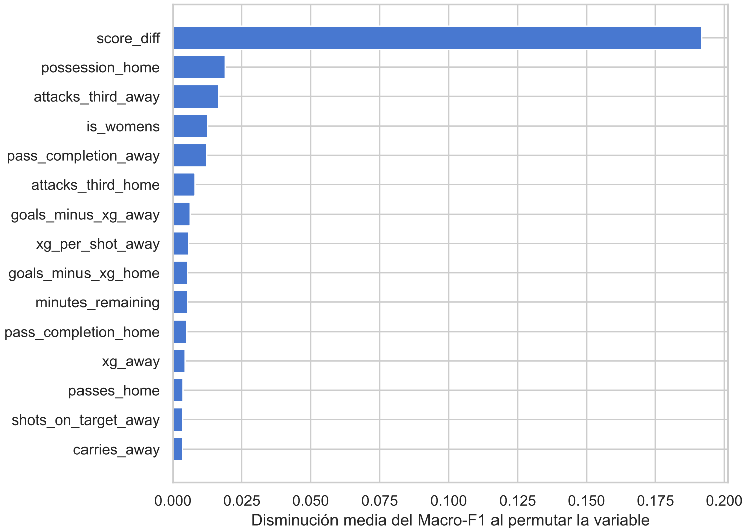
Permutation Importance - XGBoost
