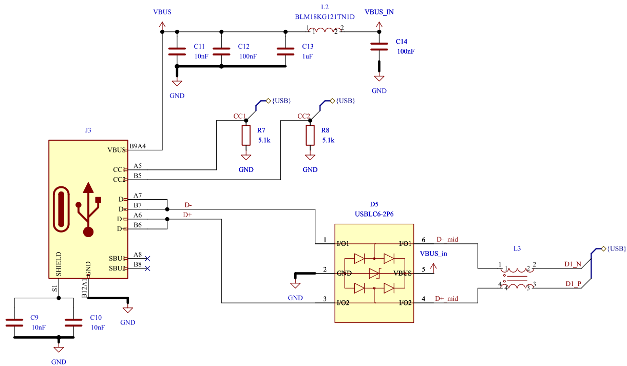
USB C Connector
