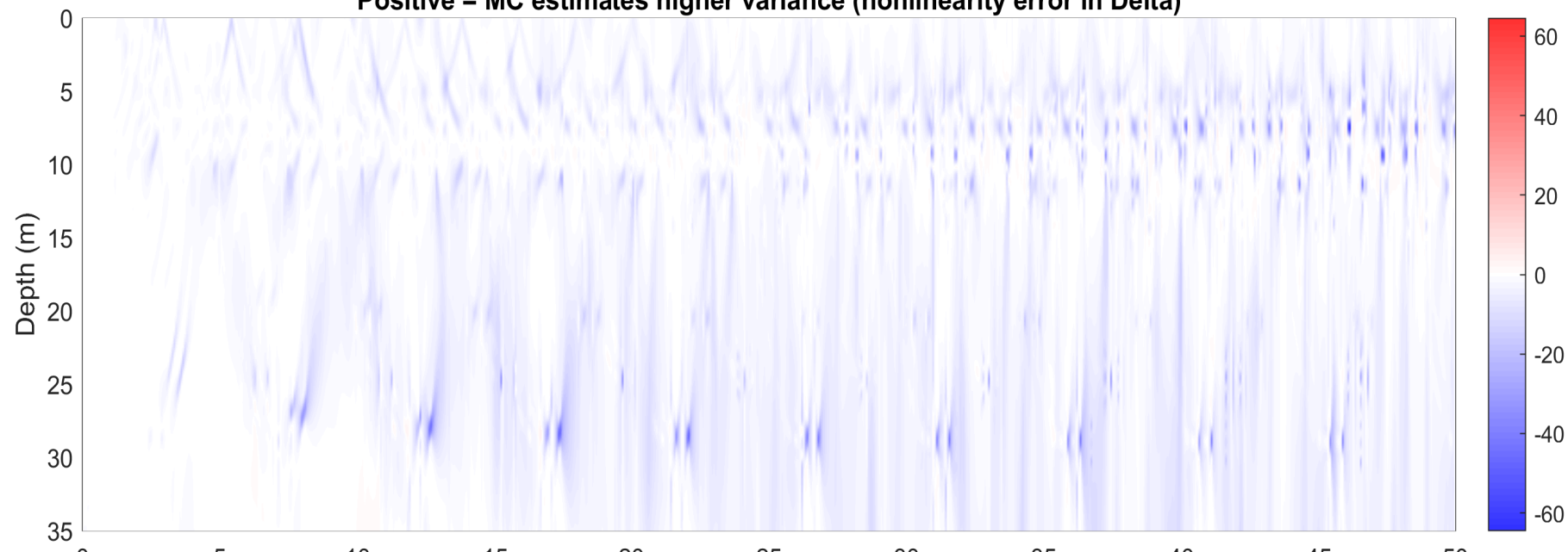
MC – Delta: Var[TL] Difference | Full 3-Param Positive = MC estimates higher variance (nonlinearity error in Delta)
