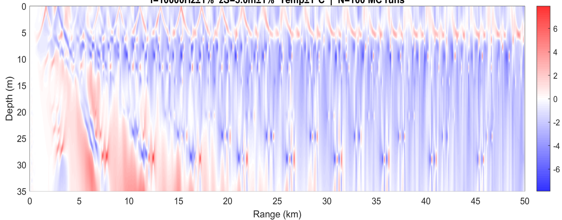
MC – Delta: E[TL] Difference [dB] | Full 3-Param f=10000Hz±1% zS=5.0m±1% Temp±1°C | N=100 MC runs
