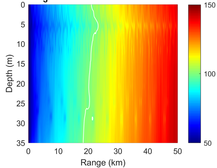
Delta E[TL] | z_S + Freq | f=10000\text{Hz} z_S=5.0\text{m} (white=FOM)
