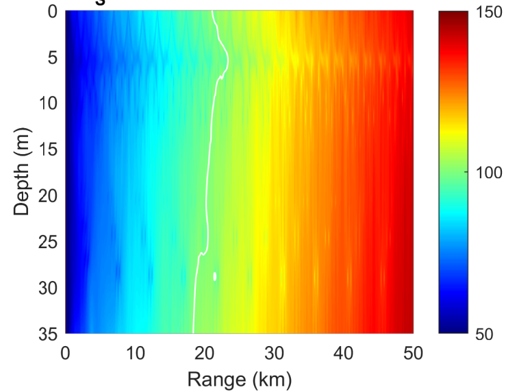
Delta E[TL] | z_S + Temp | f=10000\text{Hz} z_S=5.0\text{m} (white=FOM)
