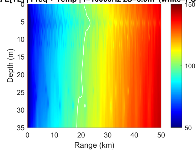
Delta E[TL] | Freq + Temp | f=10000\text{Hz} z_S=5.0\text{m} (white=FOM)
