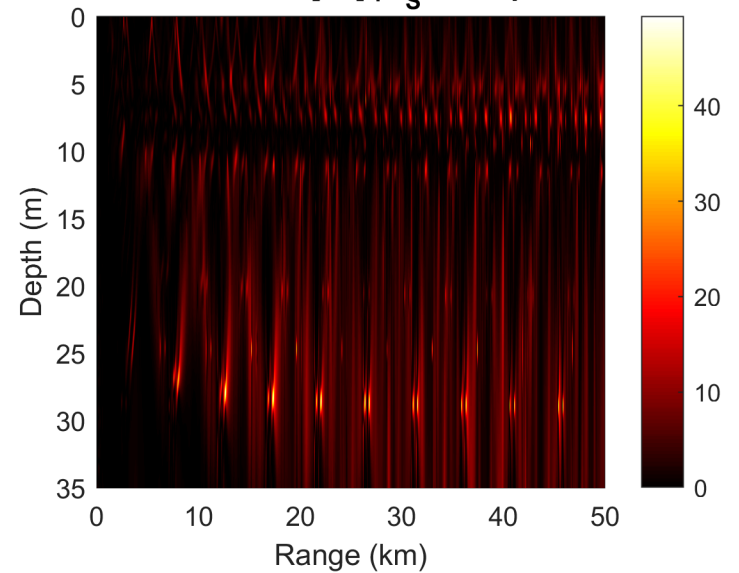
Delta Var[TL] | z_S + Freq
