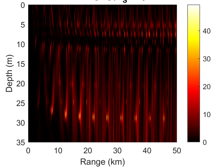
Delta Var[TL] | z_S only
