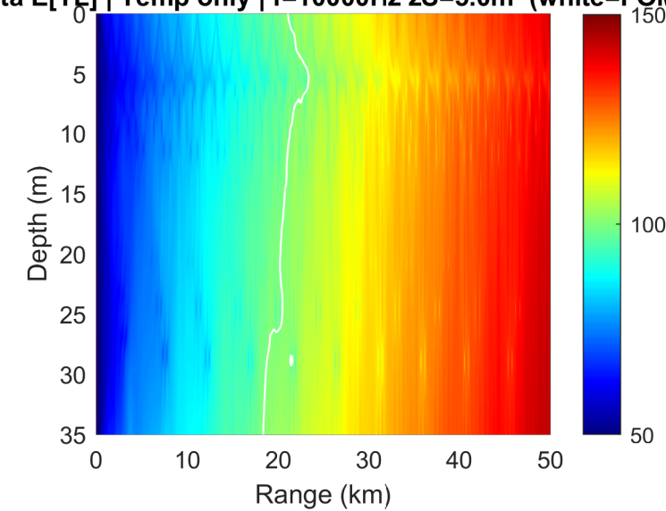
Delta E[TL] | Temp only | f=10000\text{Hz} z_S=5.0\text{m} (white=FOM)
