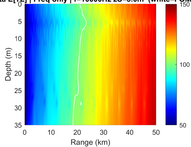
Delta E[TL] | Freq only | f=10000\text{Hz} z_S=5.0\text{m} (white=FOM)
