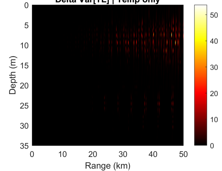
Delta Var[TL] | Temp only
