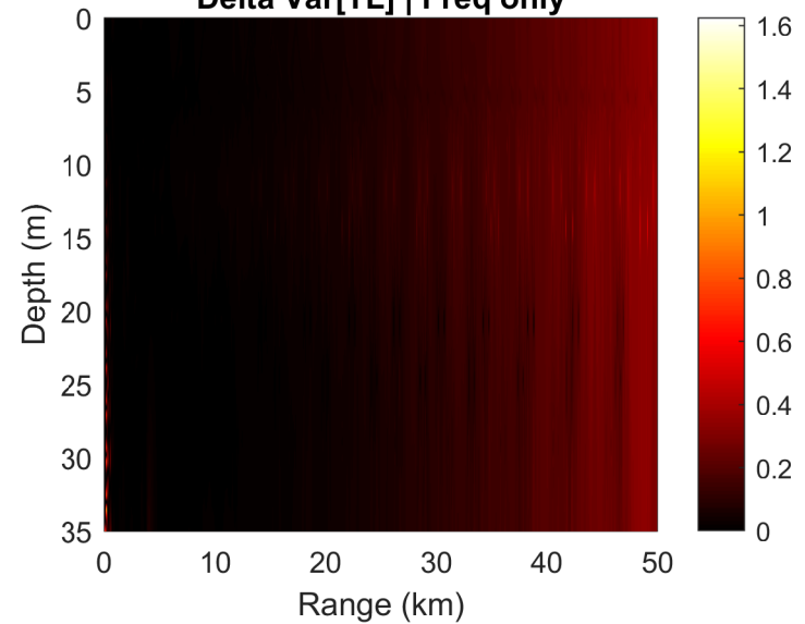
Delta Var[TL] | Freq only
