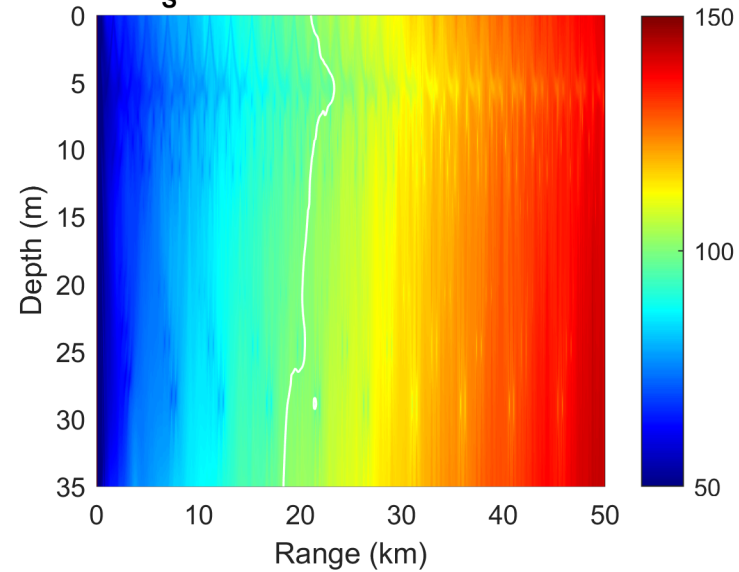
Delta E[TL] | z_S only | f=10000\text{Hz} z_S=5.0\text{m} (white=FOM)
