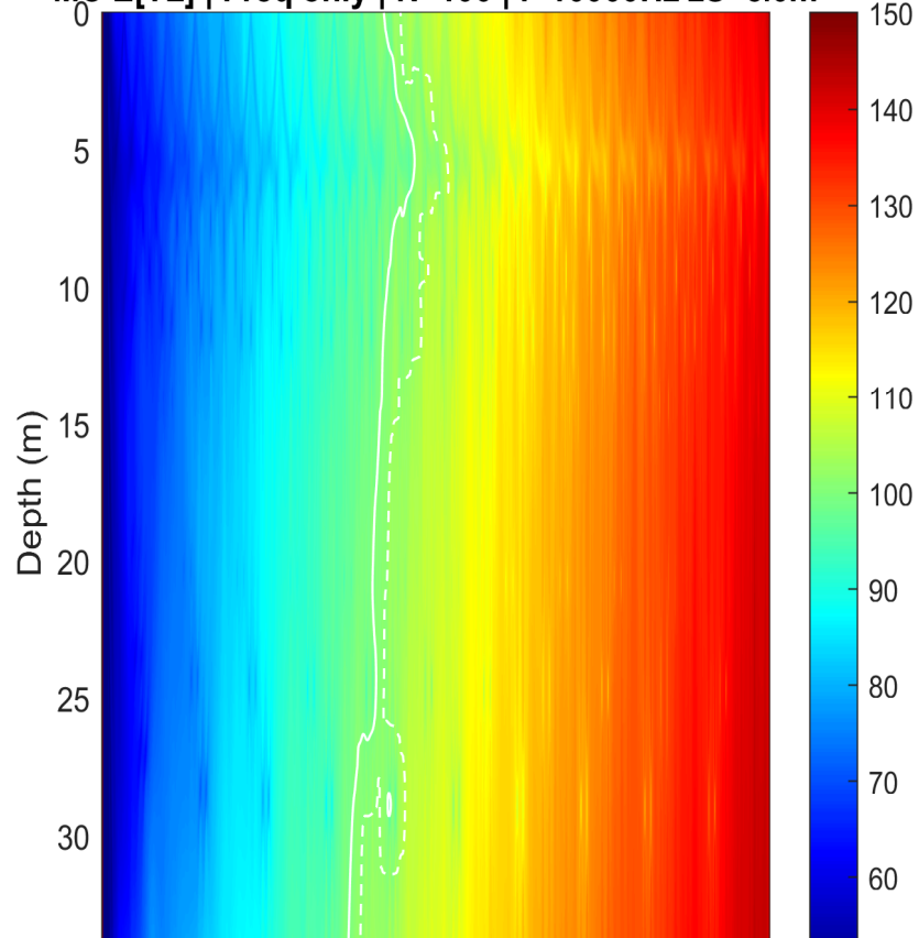
MC E[TL] | Freq only | N=100 | f=10000Hz zS=5.0m
