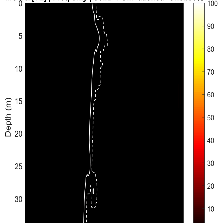
MC Var[TL] | Freq only | solid=FOM dashed=Cheb95%
