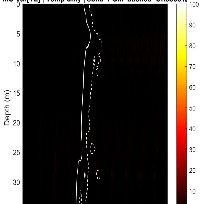
MC Var[TL] | Temp only | solid=FOM dashed=Cheb95%
