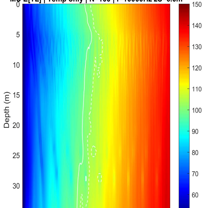
MC E[TL] | Temp only | N=100 | f=10000Hz zS=5.0m
