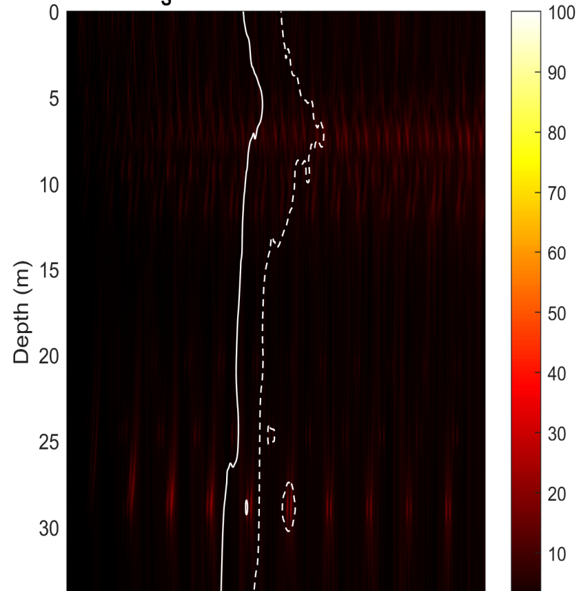
MC Var[TL] | z_s only | solid=FOM dashed=Cheb95%
