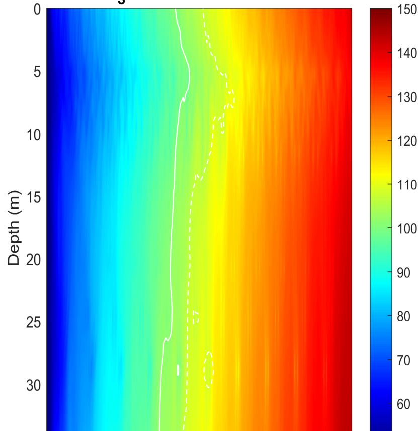
MC E[TL] | z_s only | N=100 | f=10000Hz zS=5.0m
