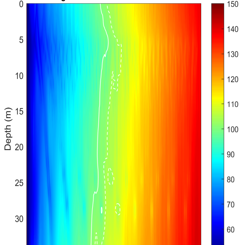
MC E[TL] | z_s + Temp | N=100 | f=10000Hz zS=5.0m
