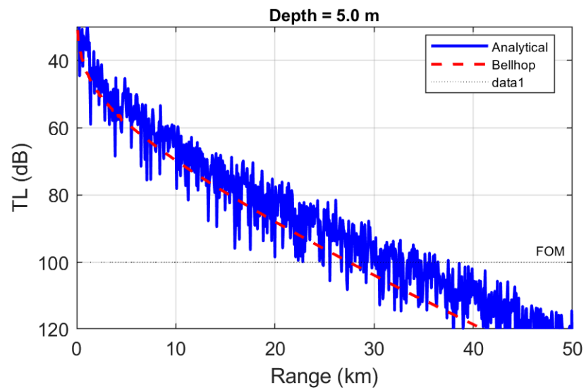
TL range profiles — Analytical (blue) vs Bellhop (red)
