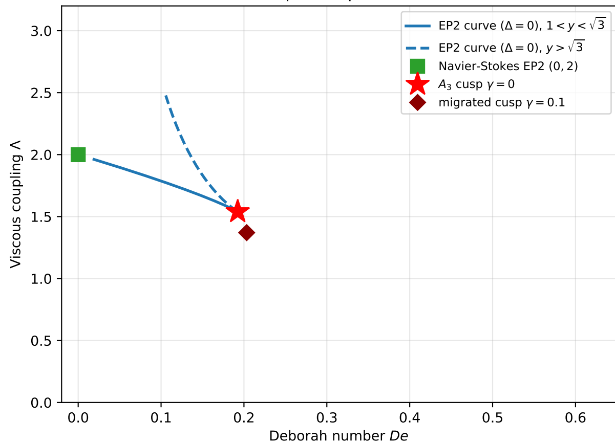
Global exceptional-point (EP2) curve
