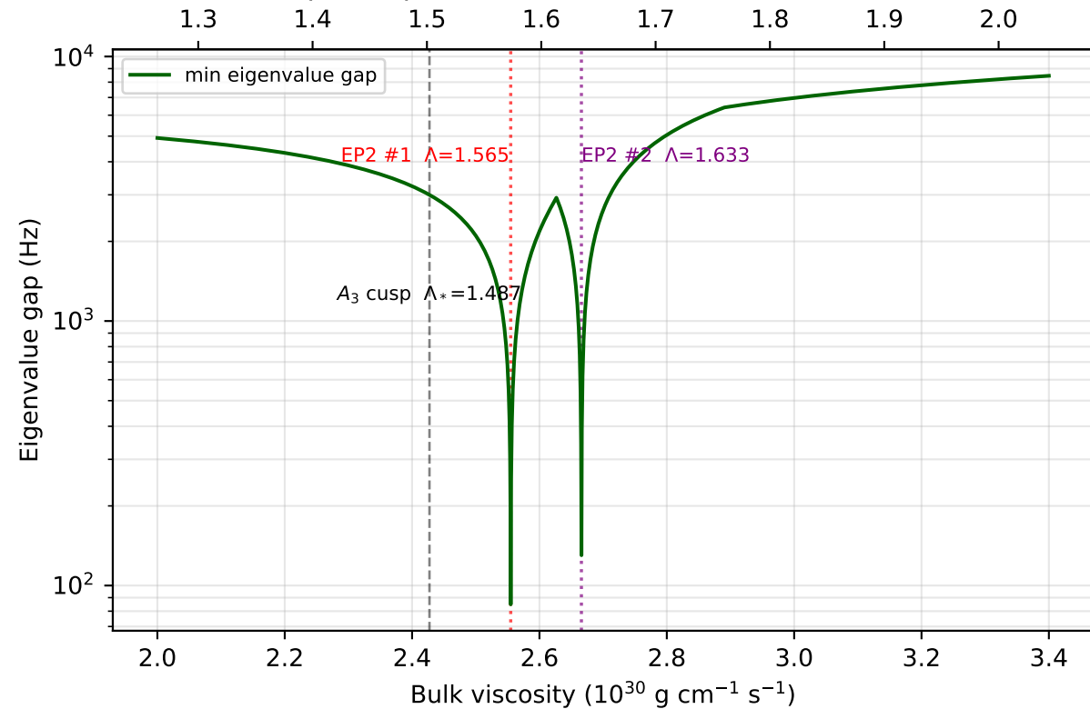
Gap collapses at both exact EP2 coalescences
