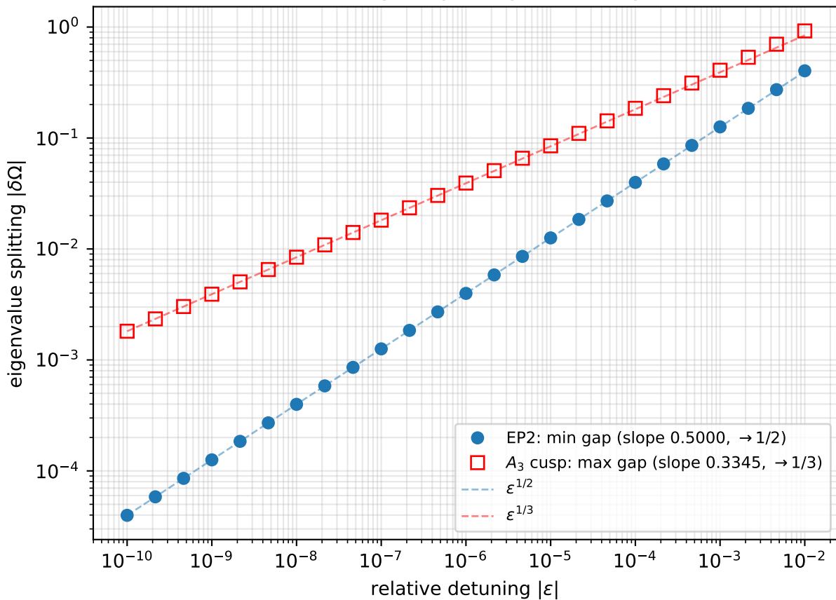
Certified non-analytic splitting at the degeneracies
