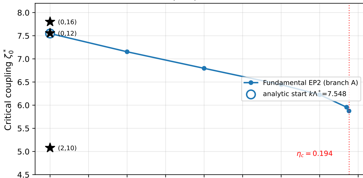
Robustness of the fundamental exceptional point under transport-profile deformation
