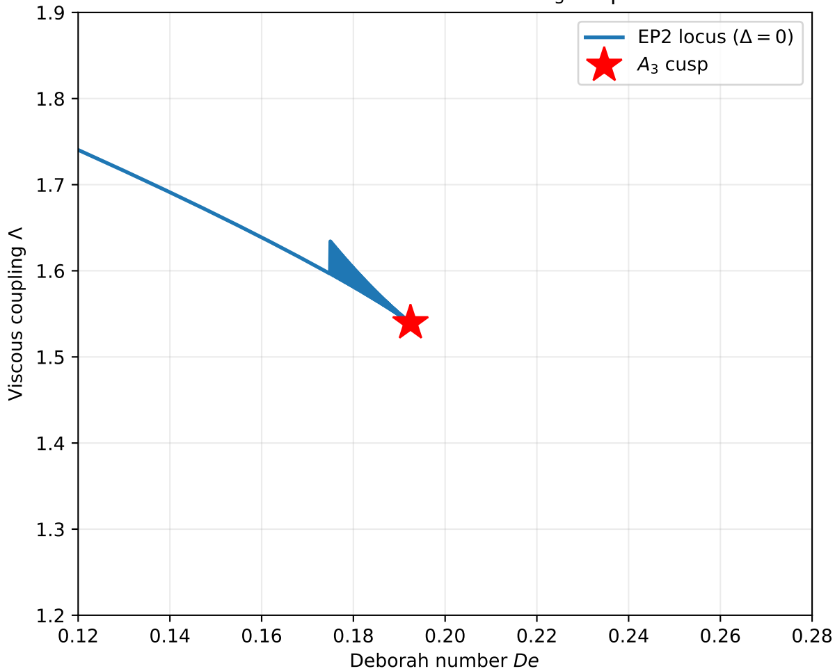
Local structure near the A_3 cusp
