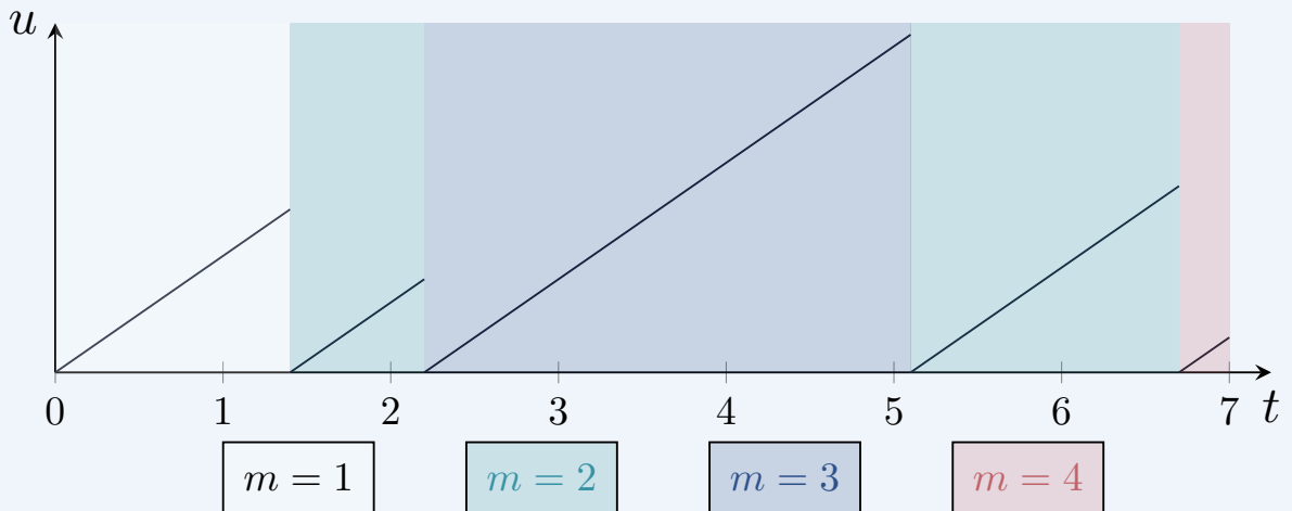
Figure 2.2: Sample trajectory of the squirrel toy example. The PDMP has a mode corresponding to the squirrel hiding place m . The Euclidean variable corresponds to the time spent by the squirrel in its current hiding place. Adapted from Amélie Vernay
