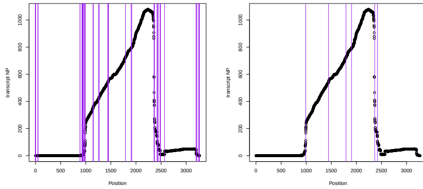
(a) Breakpoints identified by Seg-mentor3IsBack algorithm (b) Breakpoints after applying the filtering step
