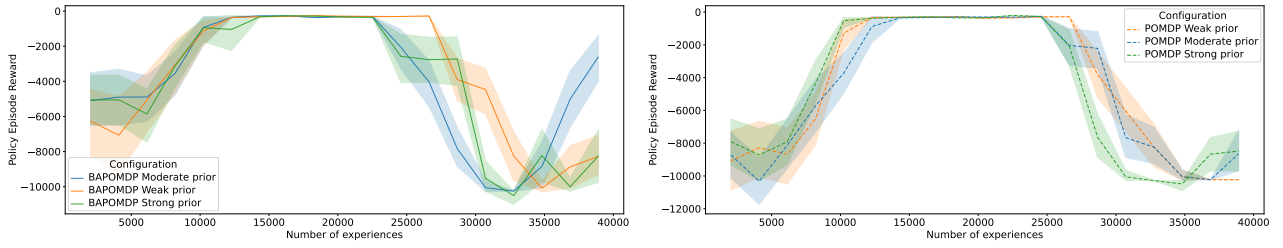
(a) Training phase with BAPOMDP model.
