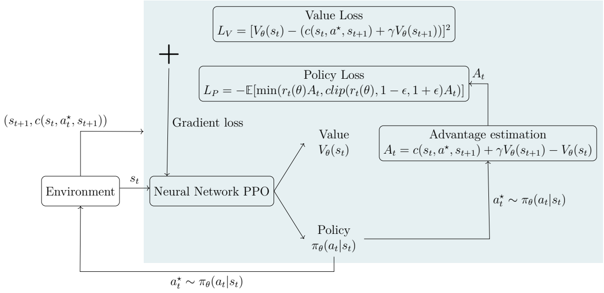
Figure 1.11: Proximal Policy Optimization algorithms. Proximal Policy Optimization (PPO) algorithms send the current state of the environment to a neural network, which calculates a probability distribution over actions (the policy) and an estimated value function. An action is sampled from the policy and executed in the environment, leading to a new state and a received cost. The collected data is then used to compute two losses: a policy loss that encourages improvement of the action distribution while constraining large policy updates with r_t(\theta) = \frac{\pi_\theta(a_t|s_t)}{\pi_{\theta_{OLD}}(a_t|s_t)} and the clip function, and a value loss that minimizes the error in value estimation. Both losses are combined, and the network weights are updated via backpropagation to progressively refine the policy and value function. In practice, neural networks process batches of transitions rather than a single state at a time, making the actual implementation significantly more efficient.
