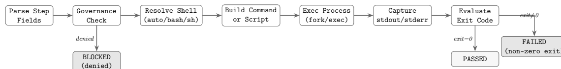
FIGURE 4.2: type: cli step execution flow: from field parsing through governance check, shell resolution, command building, process execution, output capture, and exit-code evaluation.
