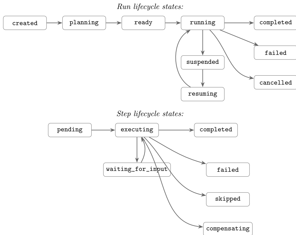
FIGURE 3.2: Execution lifecycle — run states (top) and step states (bottom).
