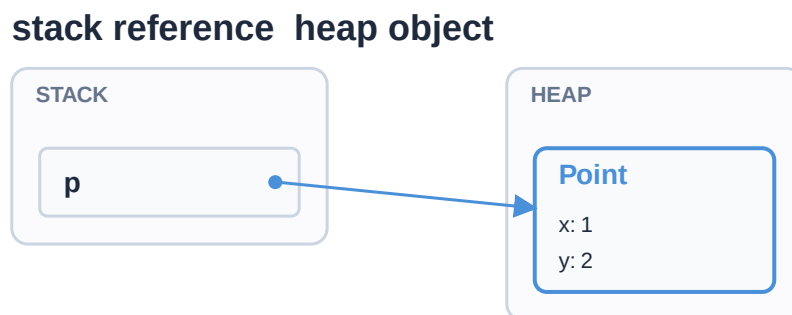
Figure 6: A memory model: a variable slot in one region holds a pointer that crosses into a heap object in another, routed by the slot-aware connector.
