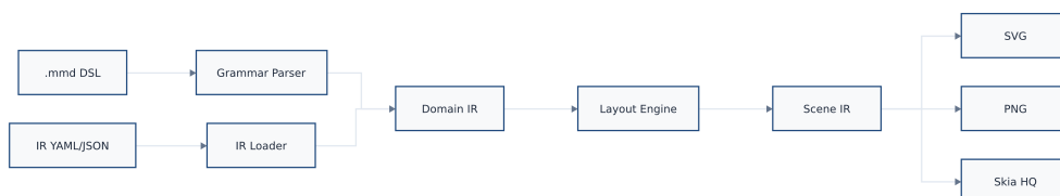
Figure 14: The two-frontend, two-IR compilation pipeline. Mermaid DSL ( .mmd ) and structured IR (YAML/JSON) both feed into a Domain IR, which the layout engine transforms into a Scene IR consumed by SVG, PNG, and Skia backends.
