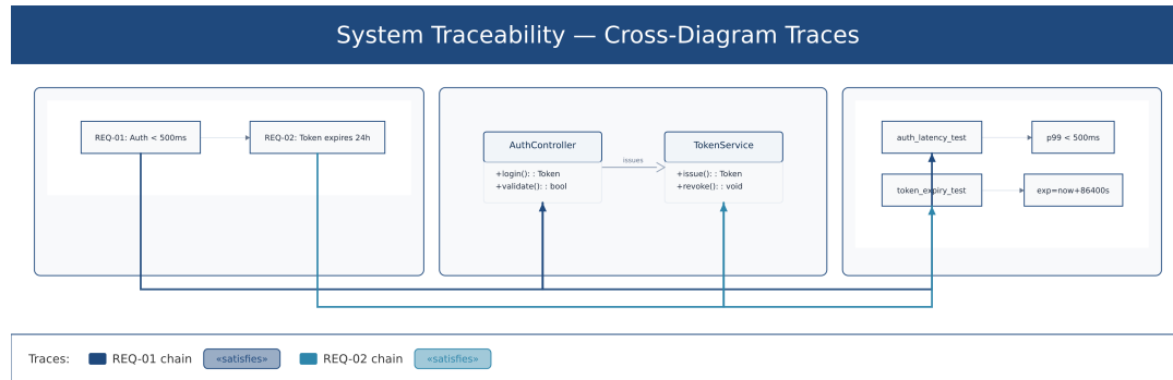
Figure 12: Rendered poster: two satisfies traces ( REQ-01 chain and REQ-02 chain ) weave a traceability thread from requirement nodes (left cell) through service classes (centre cell) to test nodes (right cell). The trace legend at the bottom shows each trace’s colour swatch, name, and !satisfies! type pill.
