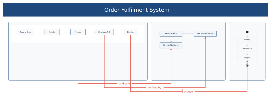
Figure 10: Rendered poster: three cross-diagram overlay edges connect the order-flow cell (left) to the service-class cell (centre) and the order-state cell (right). link edges are drawn by the compiler as directed overlay arrows on top of the composed poster grid; node positions come from the per-grammar anchor registries.
