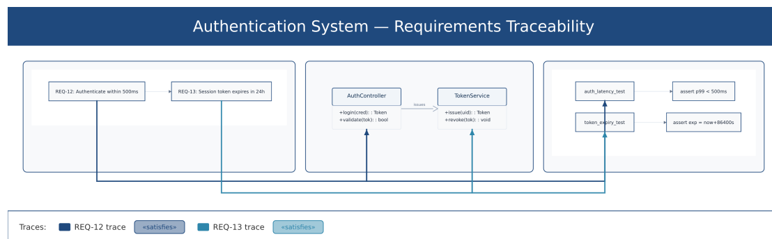
Figure 11: Rendered poster: two satisfies traces (REQ-12 trace and REQ-13 trace) weave a traceability thread from requirement nodes (left cell, flowchart) through service classes (centre cell, class diagram) to test nodes (right cell, flowchart). The auto-generated trace legend at the bottom shows each trace’s colour swatch, name, and nsatisfies type pill — rendered directly by the compiler from the listing above.
