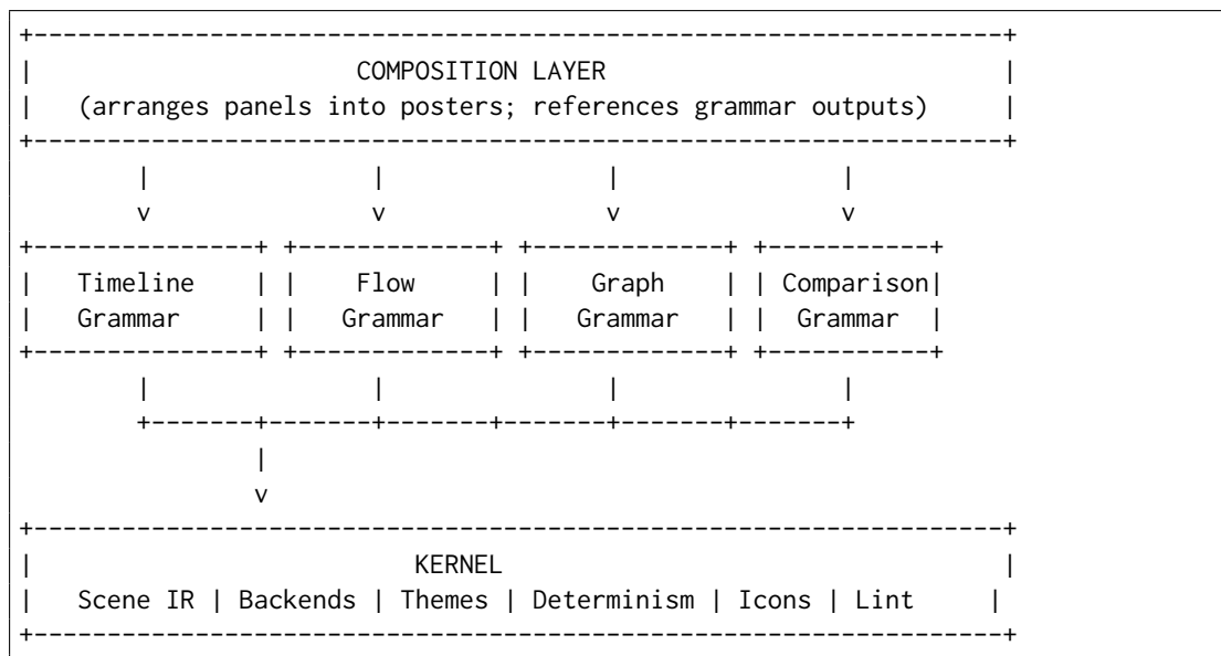
Figure 7: The three-layer architecture: Composition \rightarrow Grammars \rightarrow Kernel
