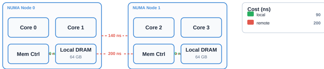
NUMA node detail
