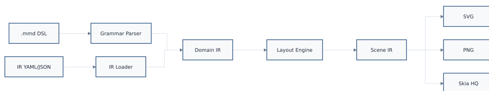
Figure 11: The two-frontend, two-IR compilation pipeline. Mermaid DSL (.mmd) and structured IR (YAML/JSON) both feed into a Domain IR, which the layout engine transforms into a Scene IR consumed by SVG, PNG, and Skia backends.
