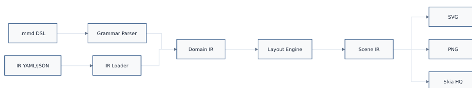
Figure 14: The two-frontend, two-IR compilation pipeline. Mermaid DSL (.mmd) and structured IR (YAML/JSON) both feed into a Domain IR, which the layout engine transforms into a Scene IR consumed by SVG, PNG, and Skia backends.
