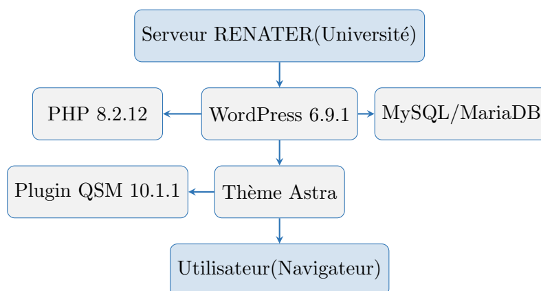
FIGURE 1 – Architecture technique du site WordPress MIAGE
