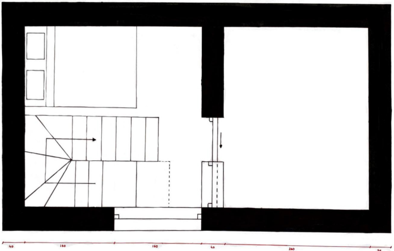
tiny house first floor plan
