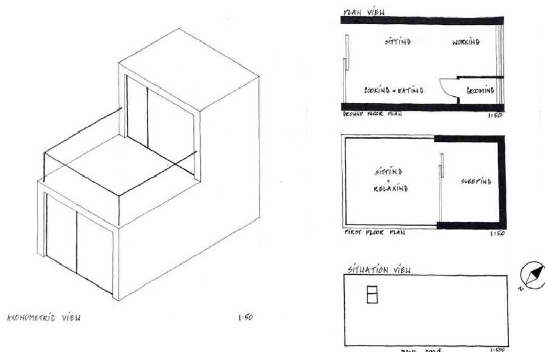
tiny house final design
