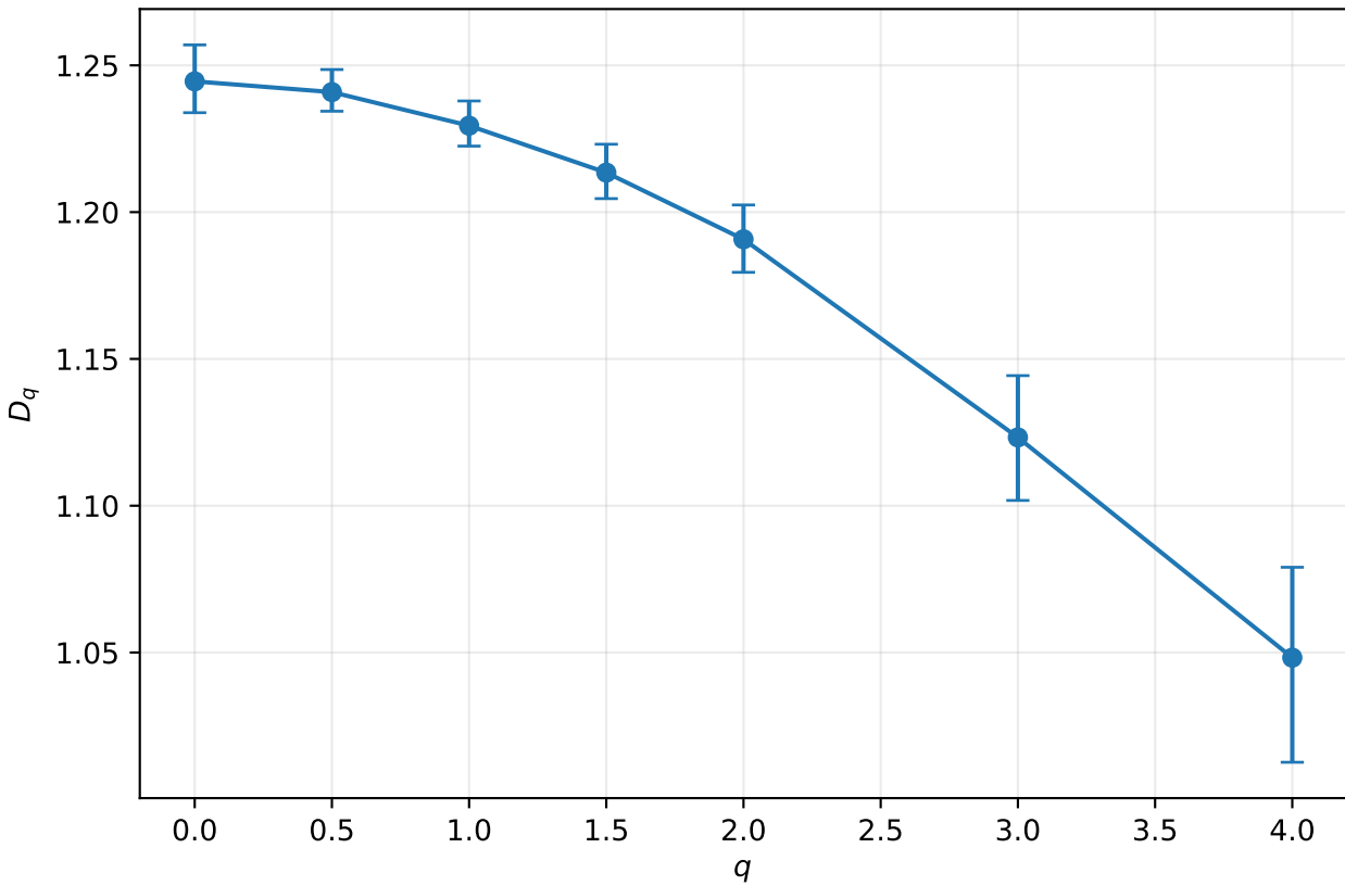
Generalised Renyi dimension spectrum
