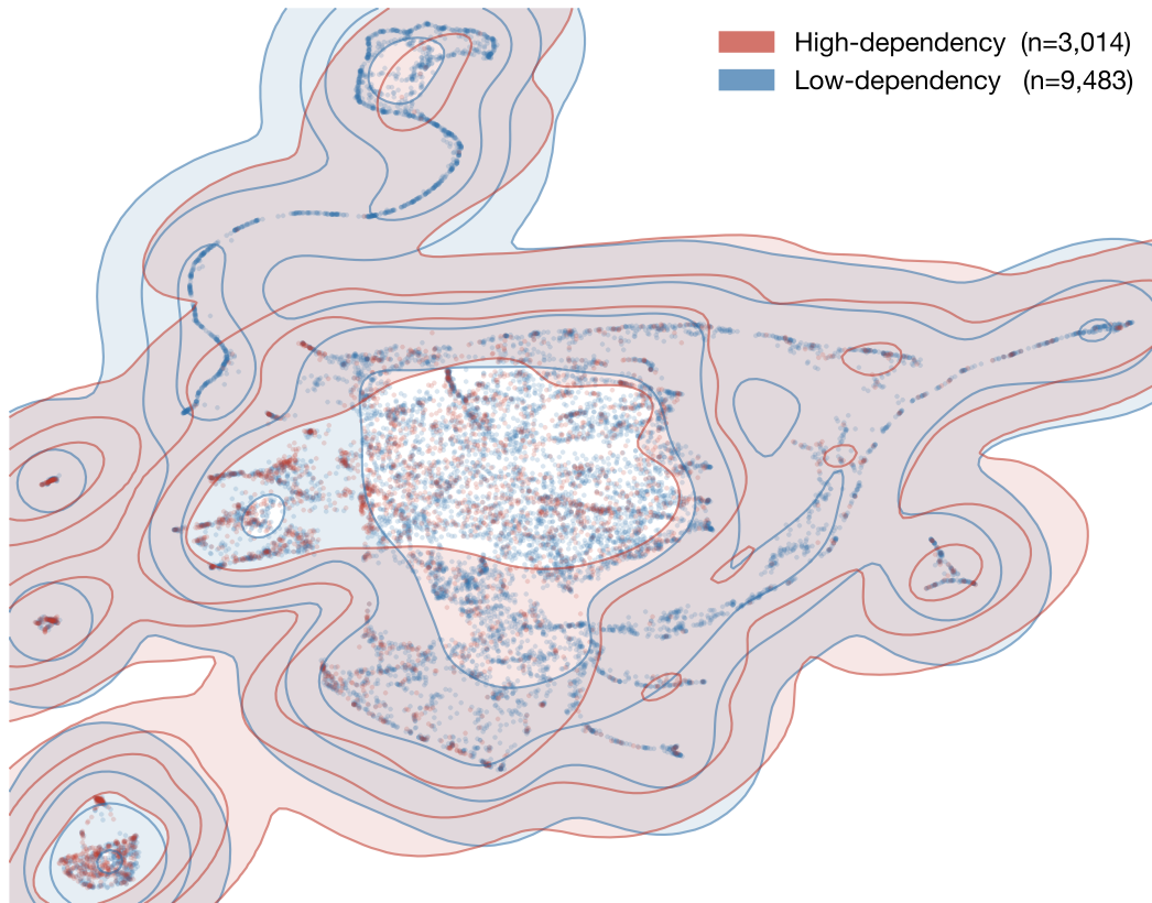
UMAP projection of early-session (sessions 1–3) feature space Contours show kernel density estimate per group
