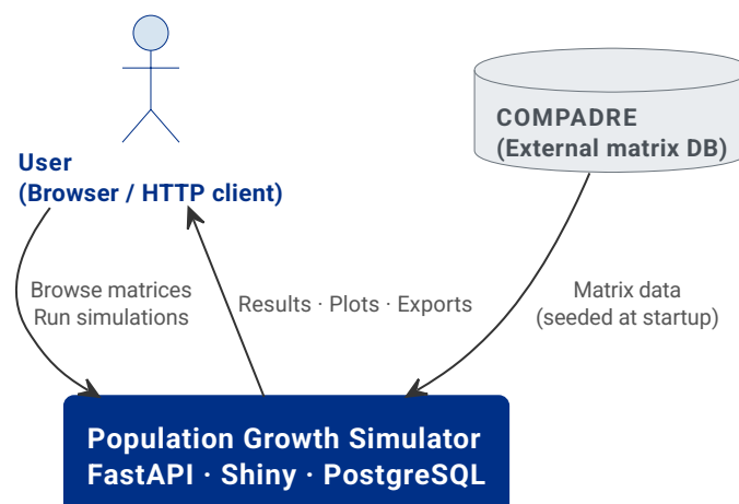
Figure 52: System context diagram. The Population Growth Simulator sits between the user's browser and the COMPADRE data source.
