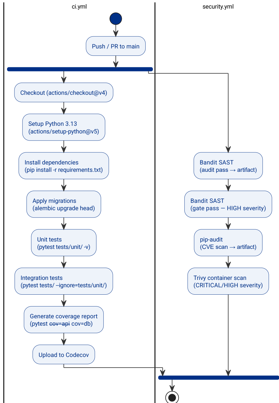
Figure 33: CI/CD pipeline. Two parallel GitHub Actions workflows handle correctness and security concerns independently.
