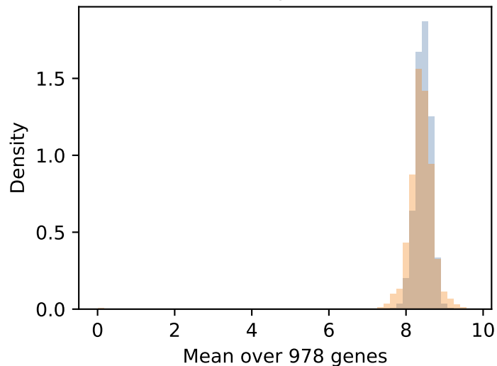
Per-sample mean
