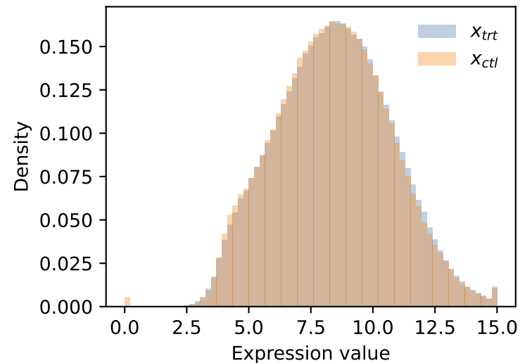
Value distribution
