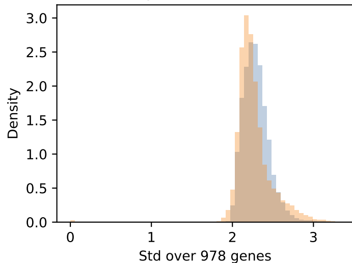
Per-sample standard deviation
