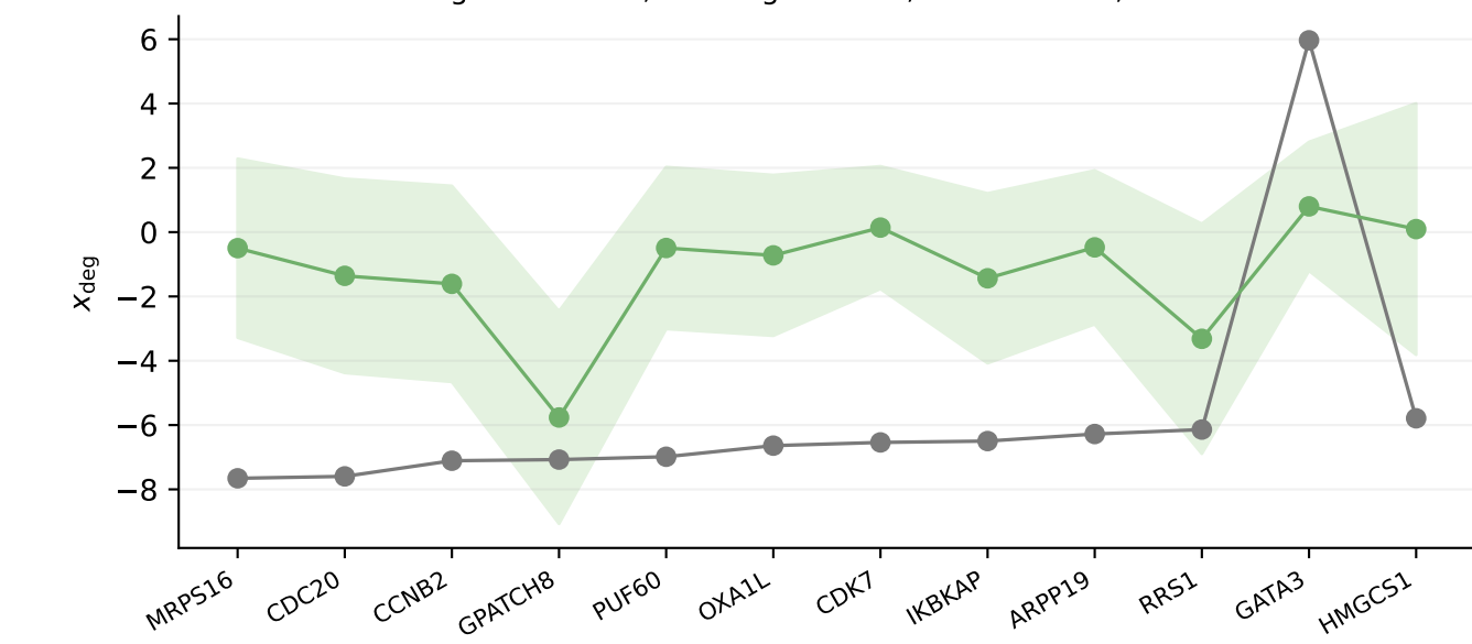
Cold cell: Higher uncertainty and larger error mean sigma = 1.146, coverage = 17%, MSE = 4.285, PCC = 0.365
