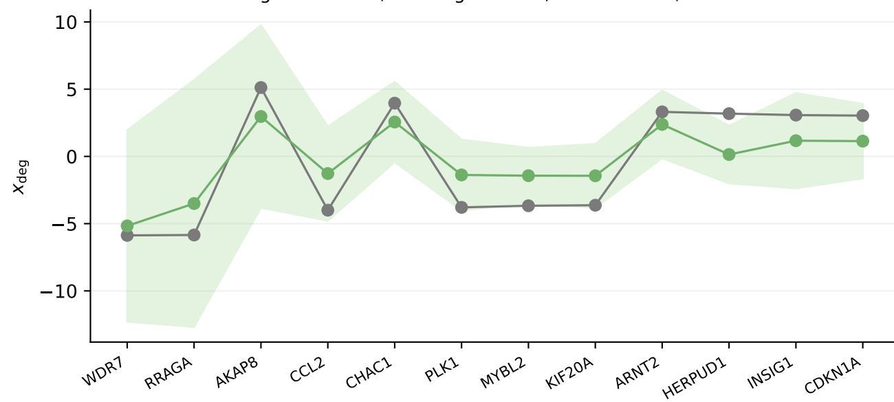
Cold cell: Lower uncertainty and better fit mean sigma = 0.760, coverage = 83%, MSE = 0.486, PCC = 0.762
