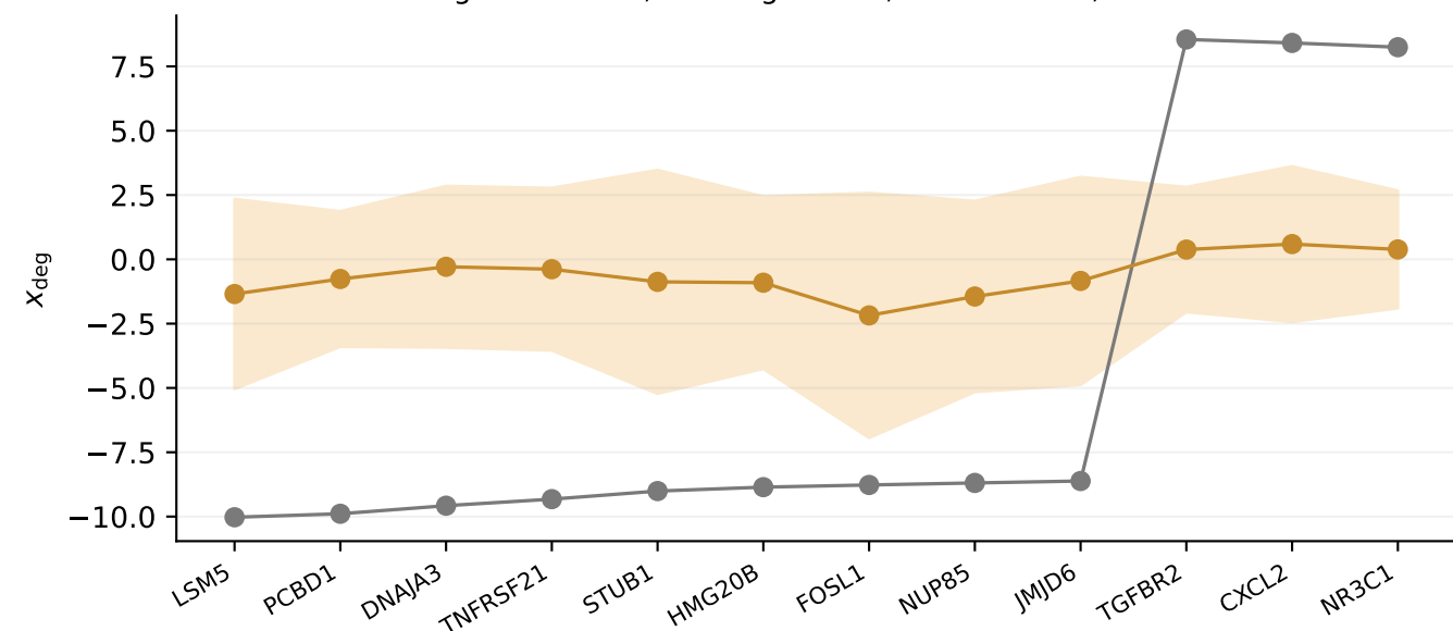
Cold drug target: Higher uncertainty and larger error mean sigma = 1.012, coverage = 8%, MSE = 9.712, PCC = 0.290
