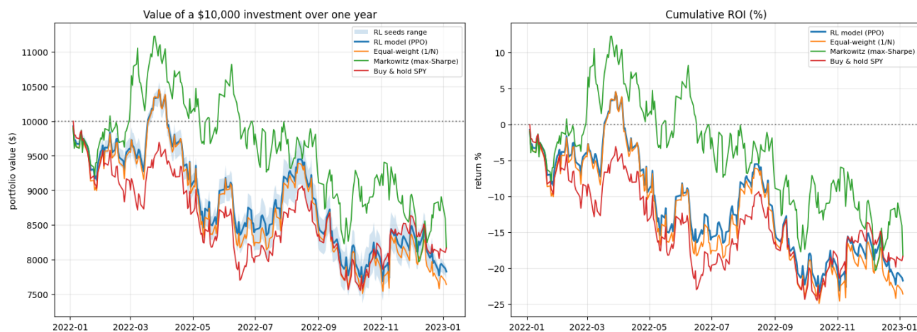
Fig. 8. A $10,000 investment over one year (2022). Left : dollar value, with the shaded band giving the spread of the PPO agent across seeds. Right : cumulative ROI. All strategies lose ground in this bear market; Markowitz ends highest.
