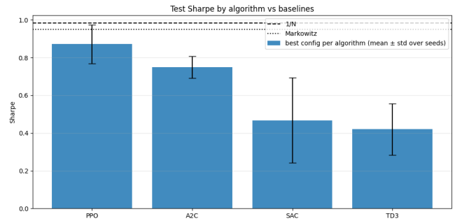
Fig. 3. Test Sharpe by algorithm (best configuration each, mean \pm std over 3 seeds) against the 1/N and Markowitz baselines (horizontal lines). PPO leads the learning methods, but both classical baselines remain above all agents.
