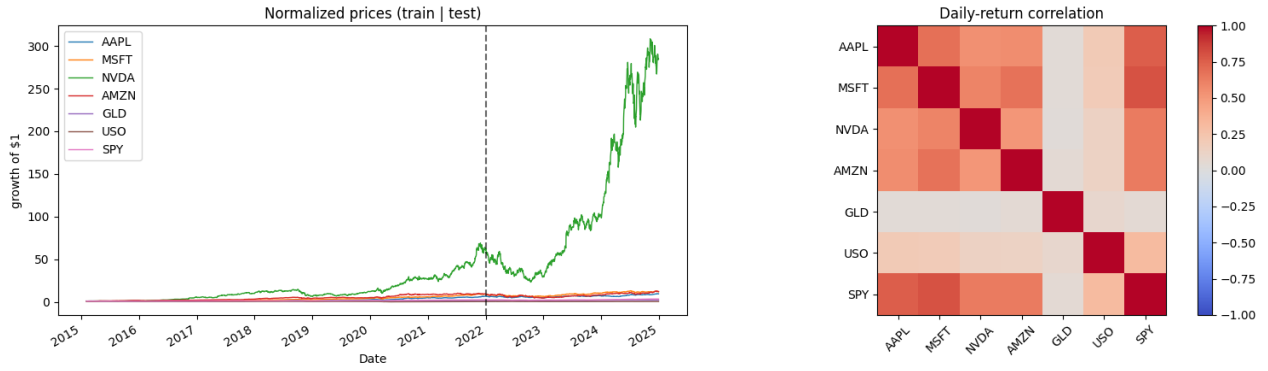
Fig. 1. Dataset. Left : normalized price paths (growth of $1) with the train/test split (dashed) at 2022-01-01; NVDA dominates the universe. Right : daily-return correlation matrix—technology names co-move strongly while GLD is nearly uncorrelated.
