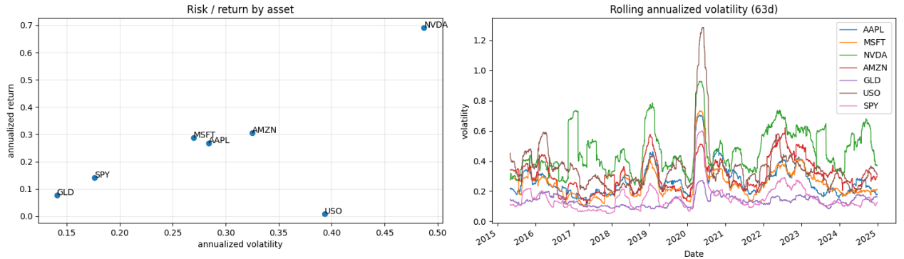
Fig. 2. Asset characteristics. Left : annualized risk/return by asset—NVDA is high-risk/high-return, GLD low-risk, USO high-risk/near-zero-return. Right : 63-day rolling annualized volatility, showing the early-2020 spike and persistent regime changes.
