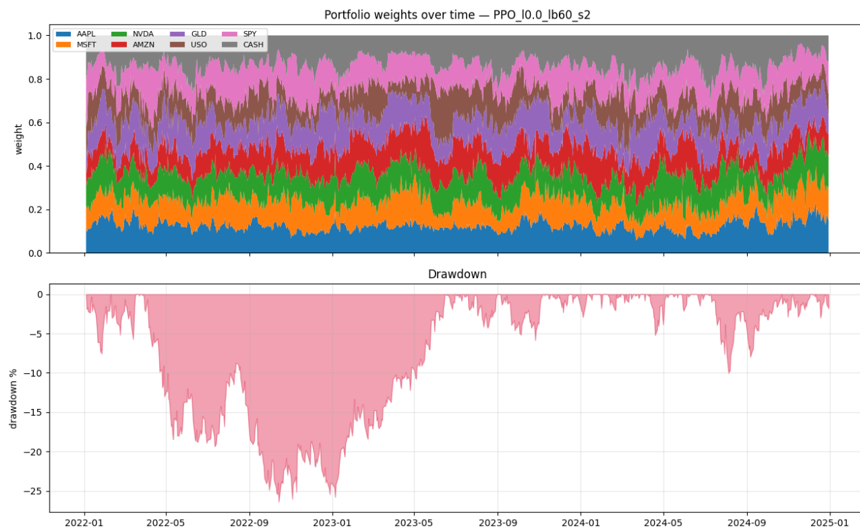
Fig. 7. Behaviour of the best PPO agent (median seed). Top : portfolio weights over time including the cash sleeve (grey), which grows during turbulent periods. Bottom : drawdown, reaching about -26\% in the 2022–early-2023 trough.
