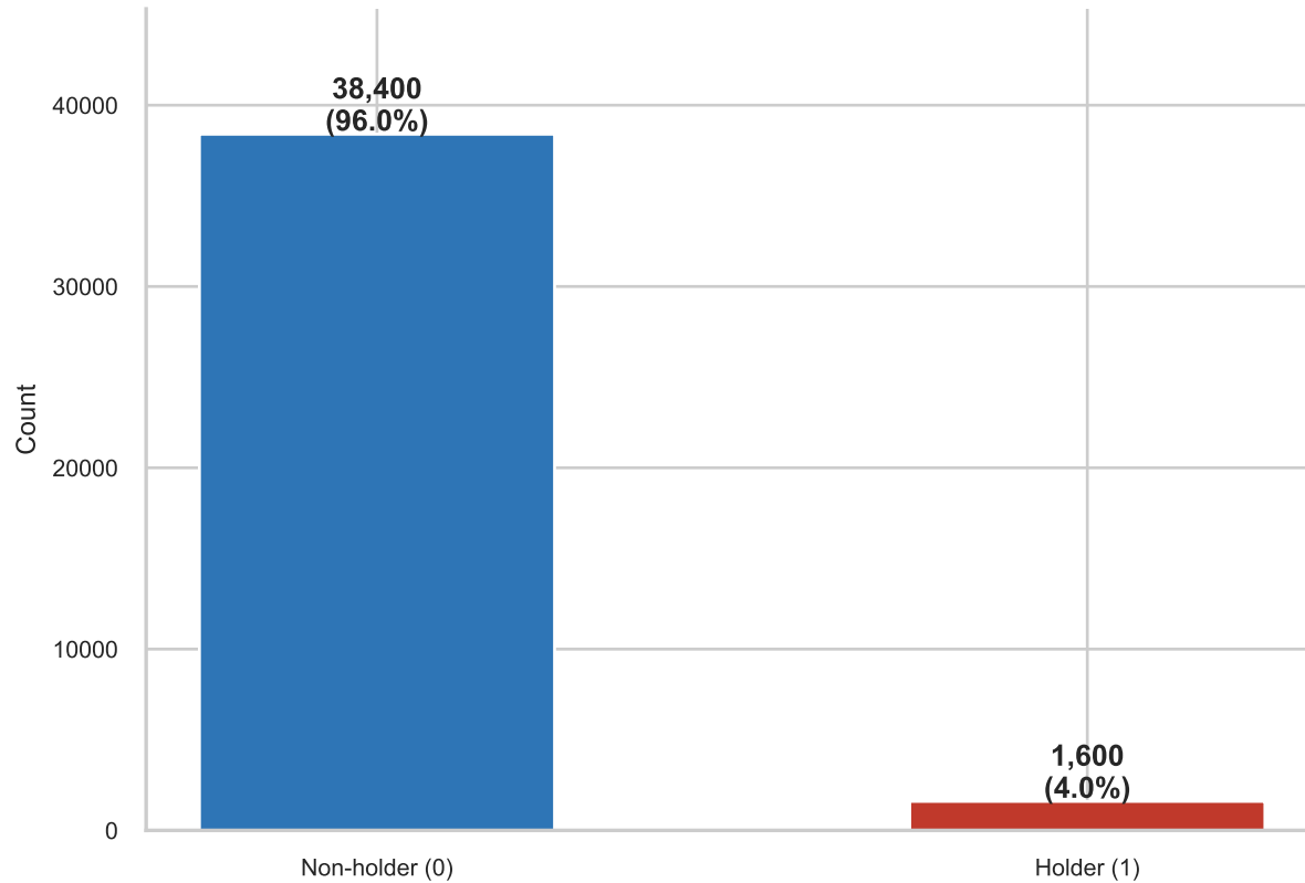
Class Counts
