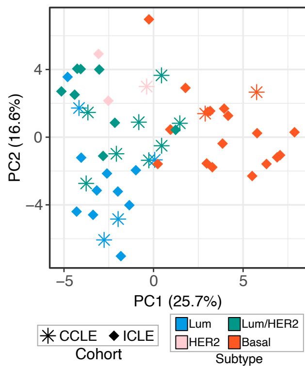
Supplementary Figure S3. Exploration of Cell Line Proteome and Definition of RPPA Subtypes.
