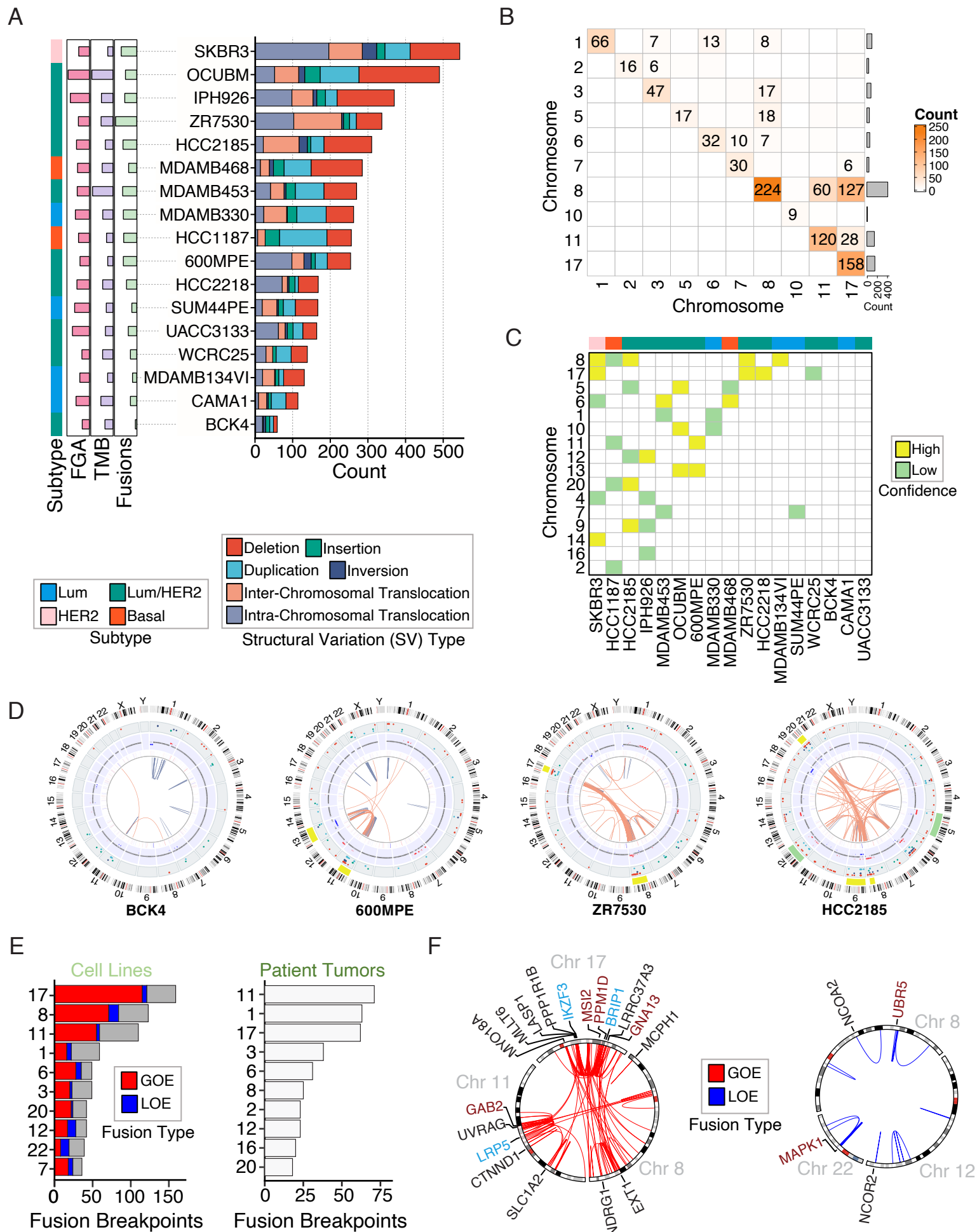
Figure 3. Optical Genome Mapping Unveils Structural Variations, Chromothripsis and Functional Fusions.
