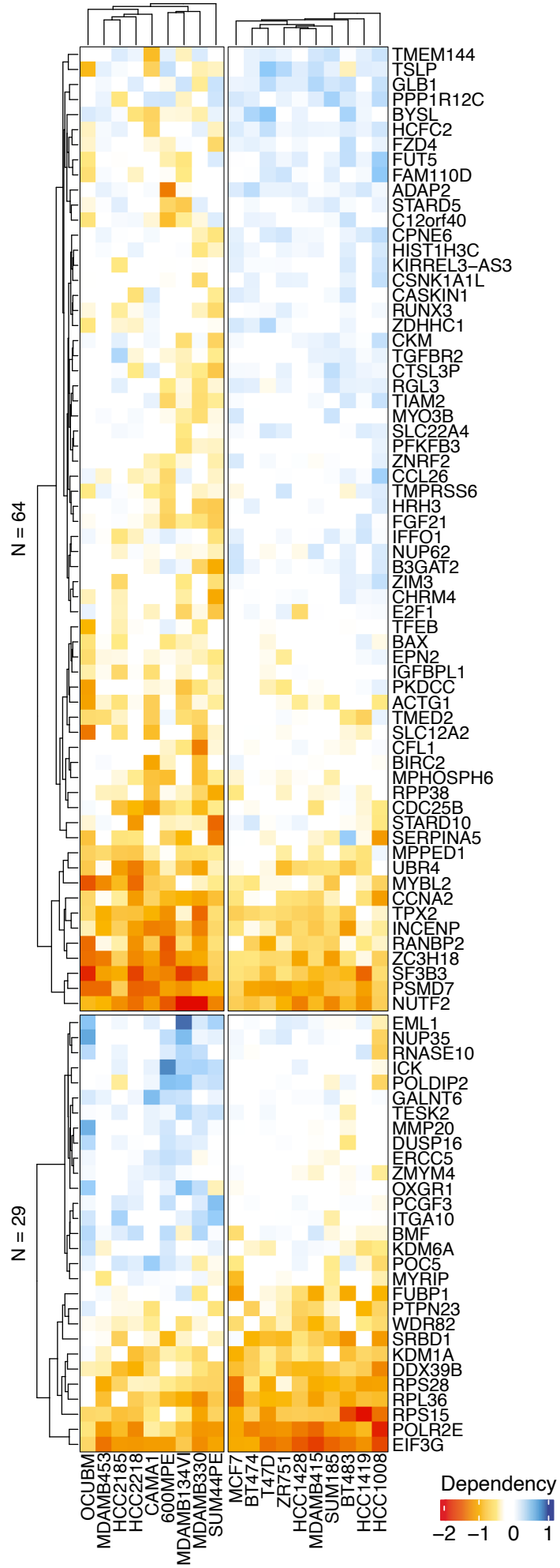
Supplementary Figure S12. Landscape of Consensus Differential Gene Dependencies.
