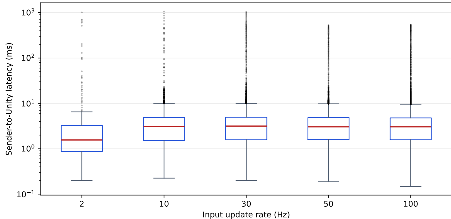
Graph 4. Latency versus input update rate
