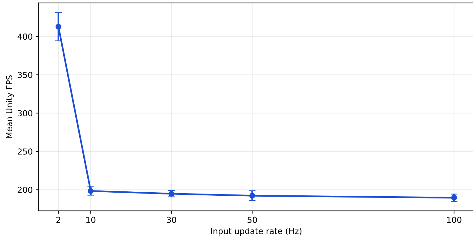
Graph 5. Unity FPS versus input update rate
