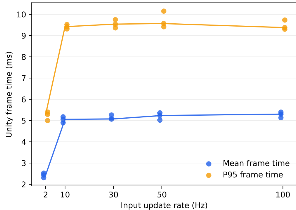
Experiment 2 frame cost under local ingestion
