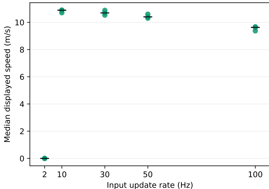
Frame-time-normalized motion
