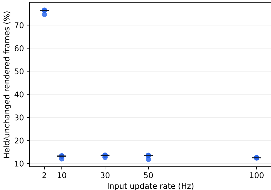
Displayed-position holds
