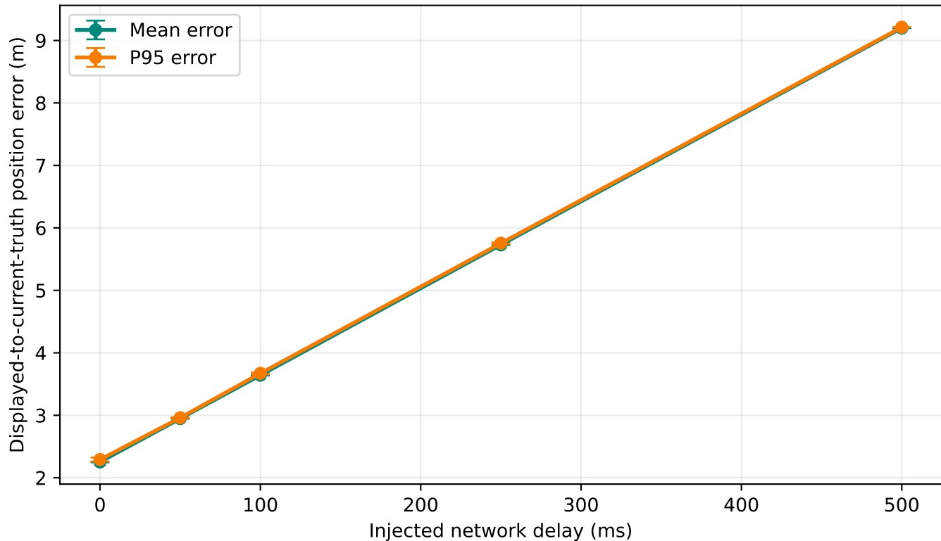
Graph 10. Position error vs network delay
