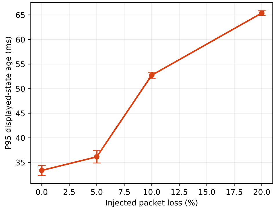
Graph 8b. State age vs packet loss
