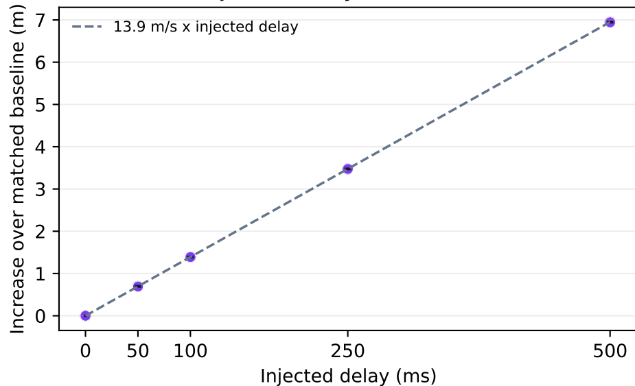
Injected-delay contribution
