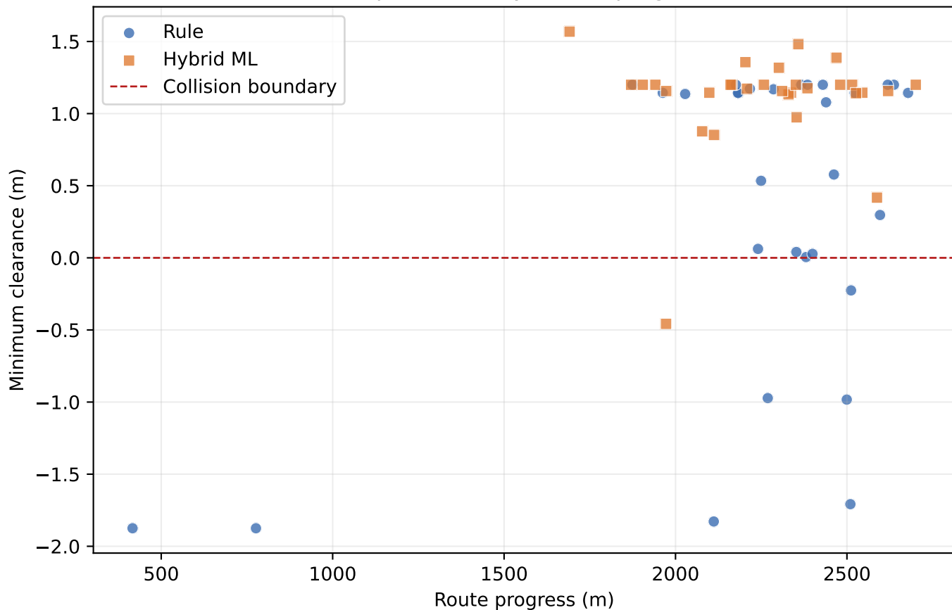
Graph 14. Safety versus progress
