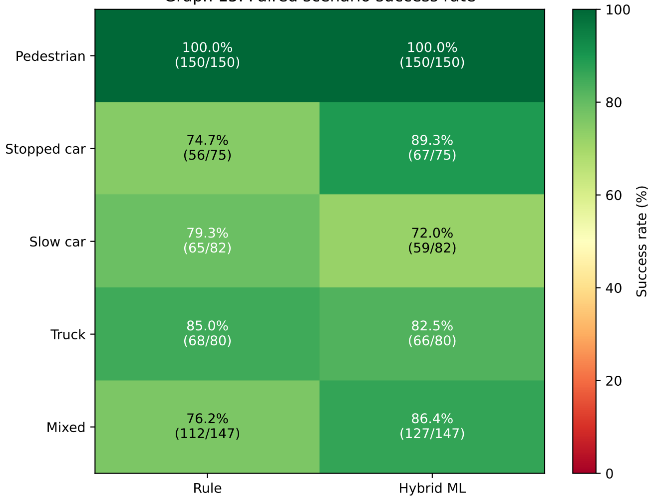
Graph 15. Paired scenario success rate
