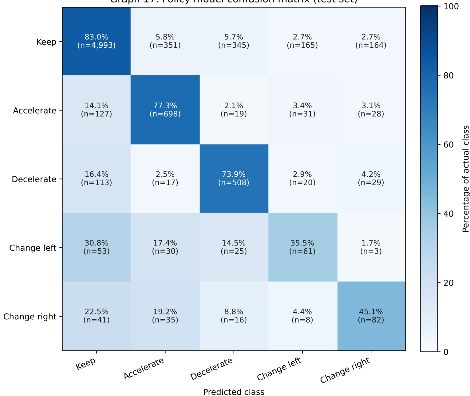
Graph 17. Policy model confusion matrix (test set)
