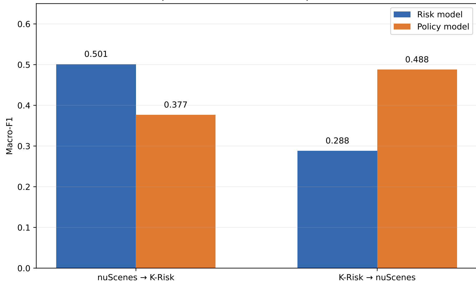
Graph 19. Cross-source transfer performance
